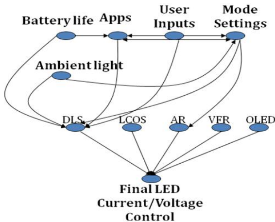
Fig. 3. New Linear Graph Representation for multilayered architecture
