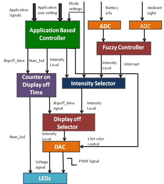
Fig. 4. Block diagram of the multilayered cross functional system
