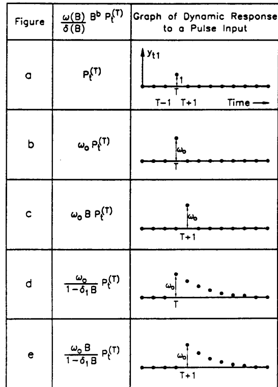
Figure 19.2.3. Dynamic response to a pulse input.
